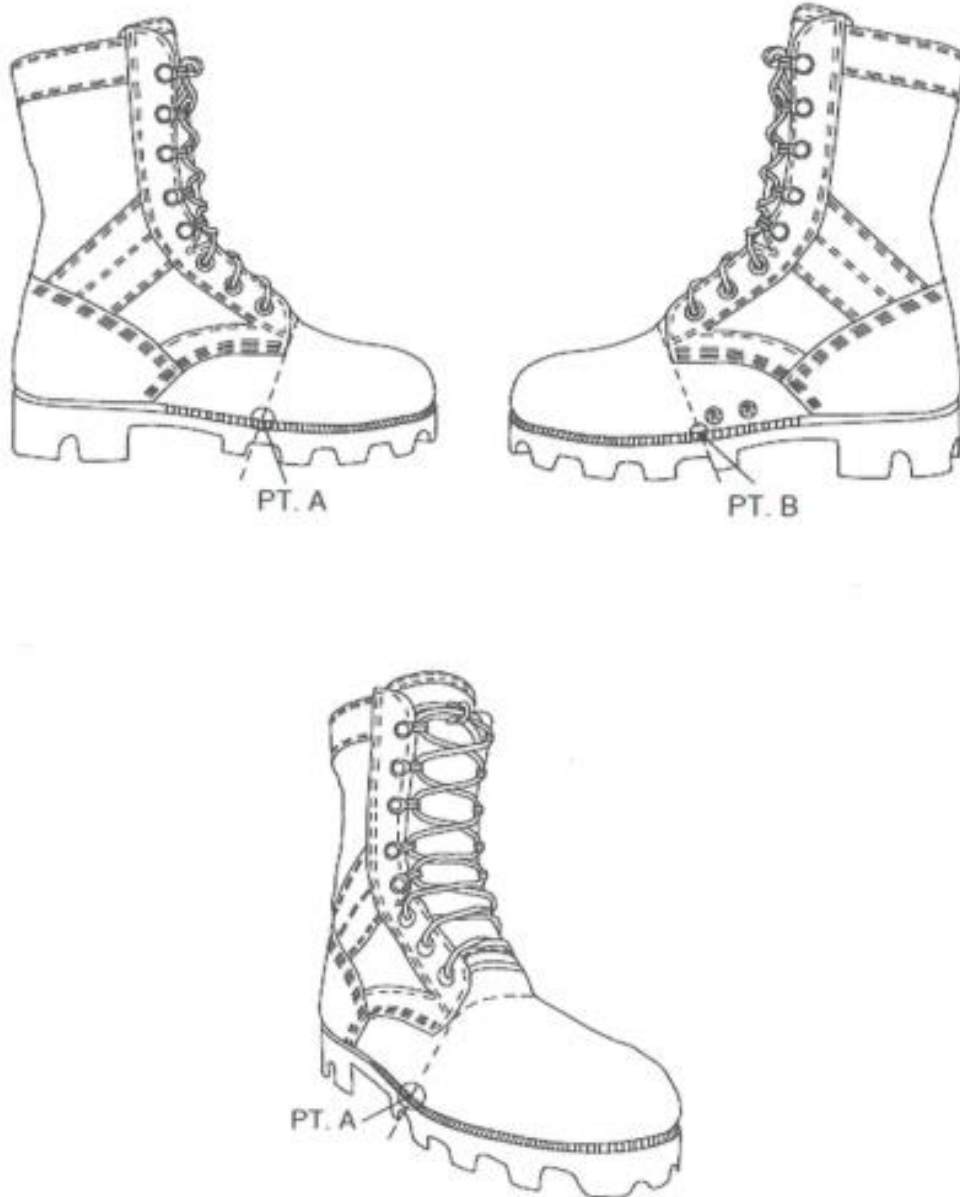
VAMP WIDTH MEASUREMENTS PT. A TO PT. B
