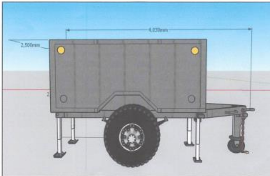
Diagram 2 - Side View
