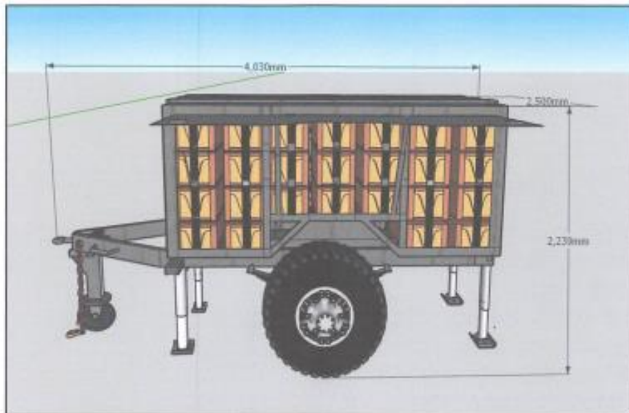
Diagram 2 - Side View
