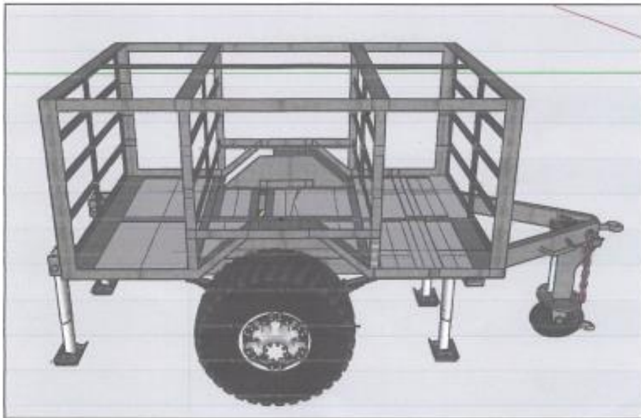
Diagram 4 – Skeletal Perspective
