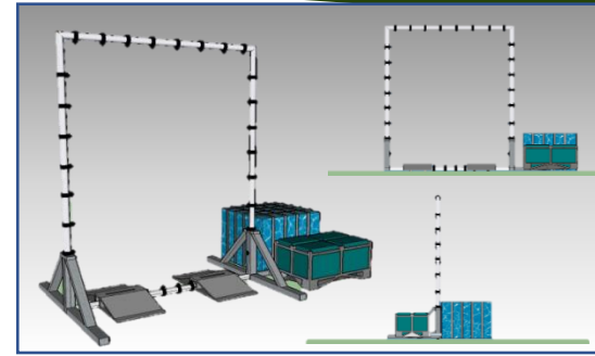
Disenyo ng RDC Vehicle Decontamination Gate
