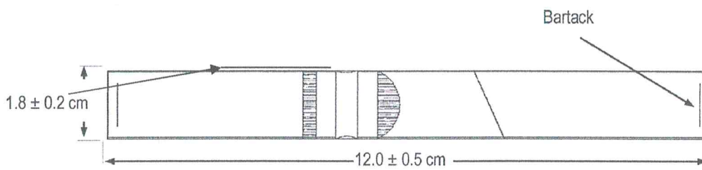
ADJUSTABLE STRAP WITH DOUBLE BAR TONGUELESS BUCKLE
