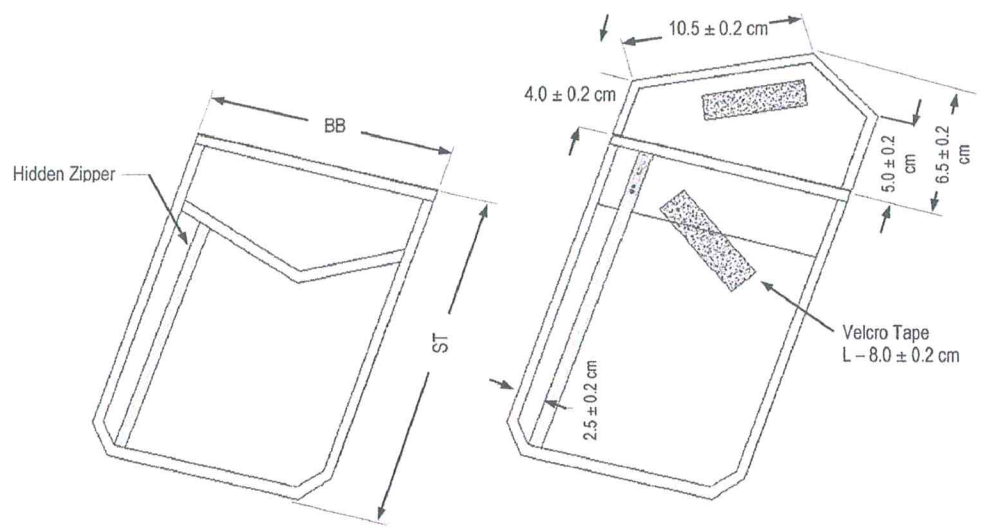
BREAST POCKET WITH FLAP
