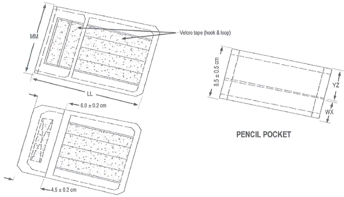
SLEEVE POCKET WITH FLAP OPEN
